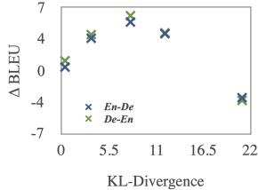
Figure 6: \Delta BLEU wrt D_{KL} . These pieces of evidence
